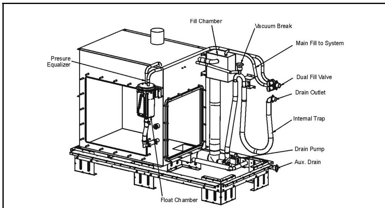
Figure 1. Humidifier Tank
