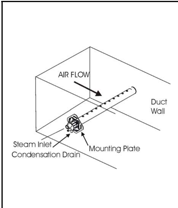
Figure 3. Steam Distributor
