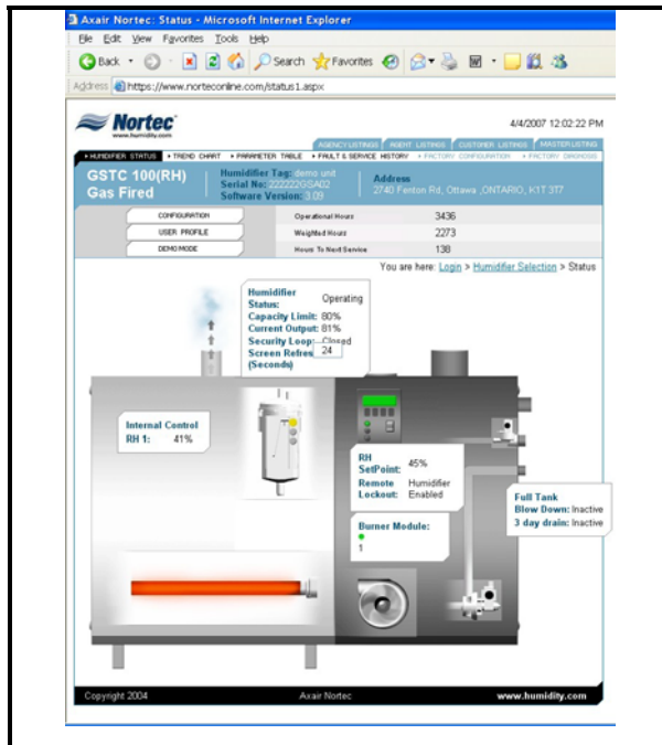
Figure 1. NORTEC Online
