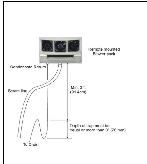
Figure 4. Blower Pack
